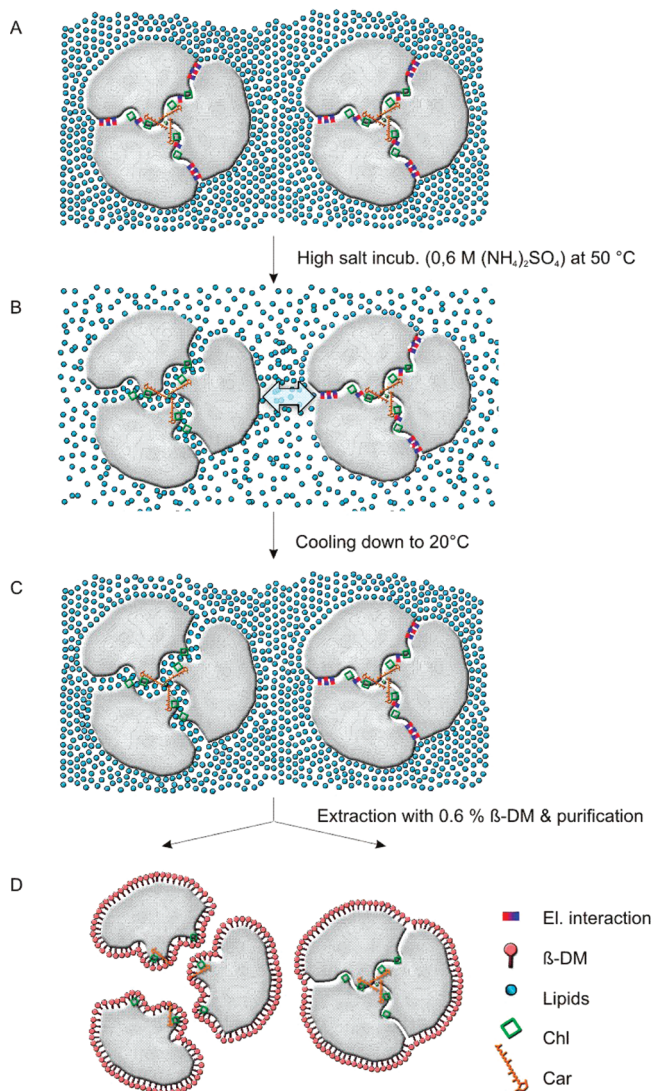
FIGURE 5: Model illustrating the experimental steps taken to monitor the equilibrium between PS1 monomers and trimers in the thylakoid membrane of T. elongatus . (A) At <30^{\circ}\text{C} (solid lipid phase), PS1 trimers are surrounded by lipids. Hydrophobic interaction (i.e., the central PsaL subunit in combination with Chl and Car) and electrostatic interaction (involving \text{Ca}^{2+} ions) may help to stabilize the trimer. (B) Heating to 50^{\circ}\text{C} (mobile lipid phase) in the presence of a high salt concentration. Weakened electrostatic interactions between PS1 monomers due to increased ion concentration. Diffusion of lipids into the PS1 trimer contact area weakens hydrophobic interactions between the monomers and establishes an equilibrium between monomeric and trimeric PS1. (C) Cooling to 20^{\circ}\text{C} (solid lipid phase). PS1 monomers and trimers are surrounded by lipid molecules ("trapped equilibrium"). (D) Lipids of extracted PS1 complexes are replaced by the detergent \beta -DM. Due to the pre-separation of monomeric PS1 in the thylakoid membrane, the isolation of intact PS1 monomers is possible; additionally, preexisting PS1 trimers are isolated.
